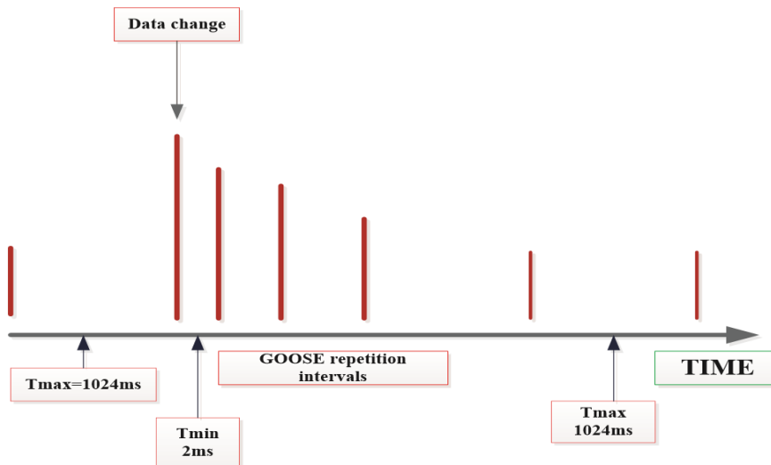
Figure 1. Reliability of the GOOSE message
