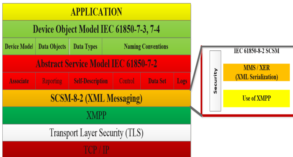
Figure 12. Protocol Stack for IEC 61850-8-2
