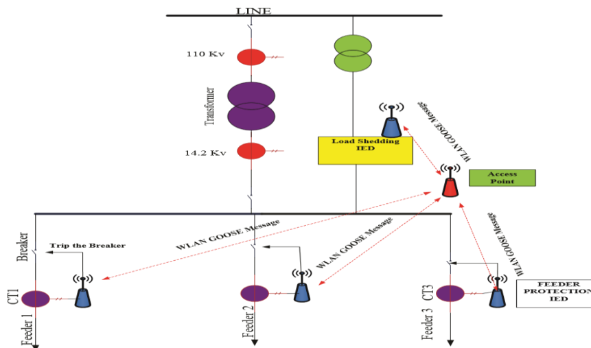
Figure 5. Centralized shedding based on wireless LAN
