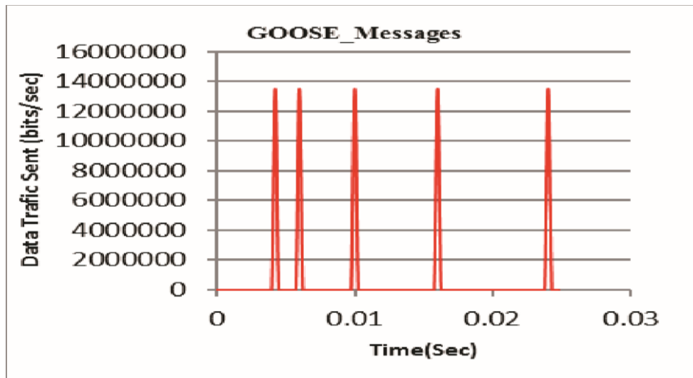
Figure 3. GOOSE message from Fault Feeders
