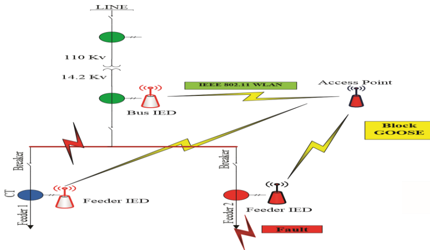
Figure 6. The concept of the fast distribution bus protection scheme
