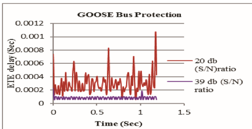
Figure 7. ETE GOOSE Message for Fast Bus protection
