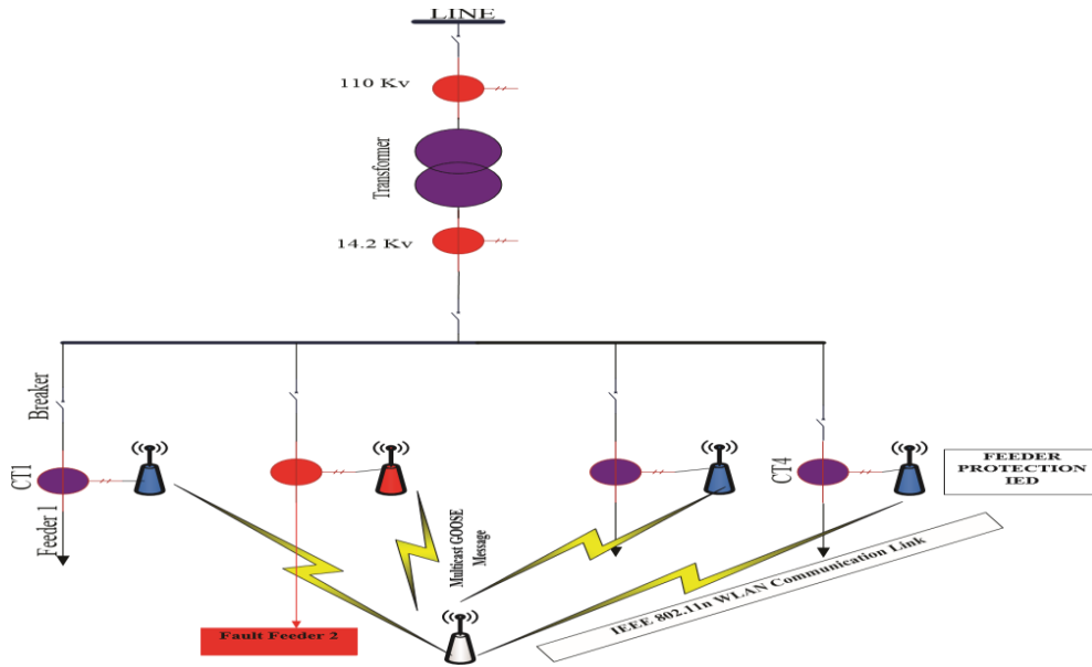
Figure 2. GOOSE message for fault feeder's distribution
