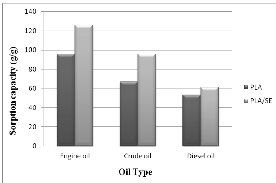
Figure 4. Oil sorption capacity of fiber samples for oils used
