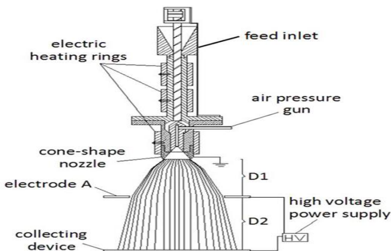
Figure 2. Schematic of the melt differential electrospinning device
